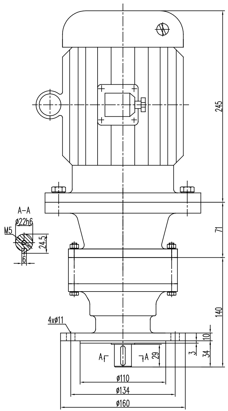
BLD09-0.55kW 立式直联型摆线针轮减速机 NER GROUP CO.,LIMITED www.sogears.com
