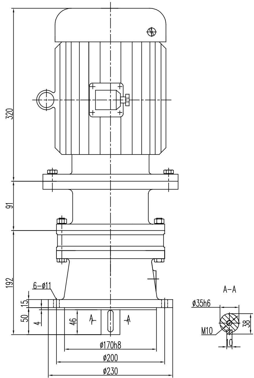
XLD3-2.2~3kw NER GROUP CO.,LIMITED 立式电机接盘型摆线针轮减速机 www.sogears.com
